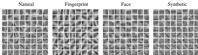
Figure 1: ICA bases from natural, fingerprint, face, and synthetic images.
